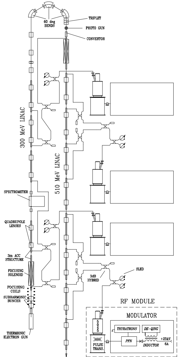
Fig. 1: General scheme of the preinjector.
