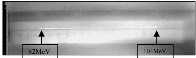
Fig.6. Accelerated beam with RF buncher switched off.
