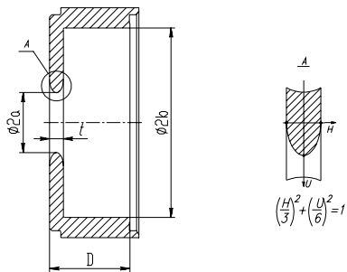
Fig. 2. Geometry of accelerating section's cell.
