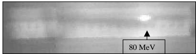
Fig.7. Accelerated beam with RF buncher switched on.
