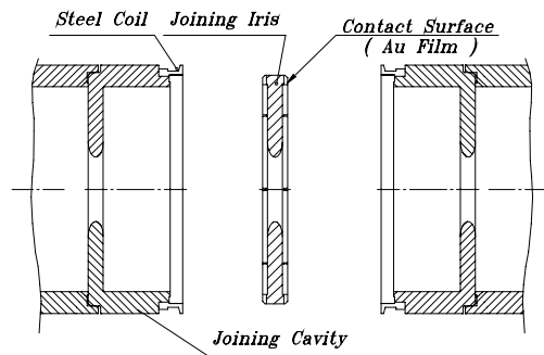
Fig. 3. Connection of two AS parts.
