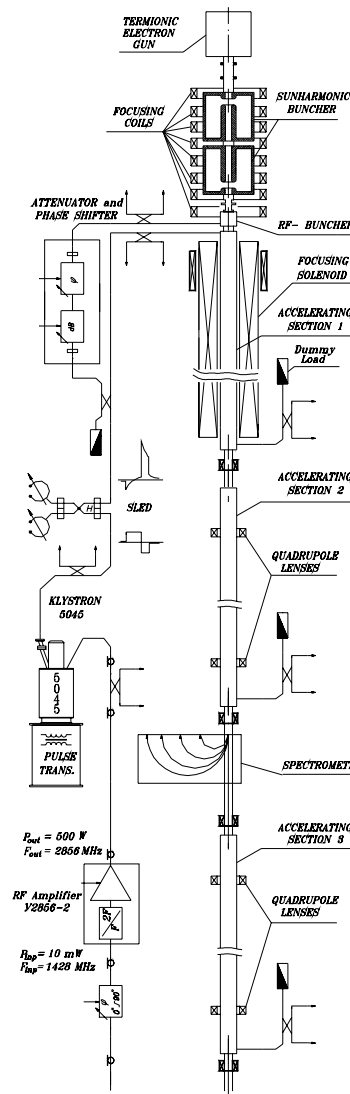
Fig.1 The scheme of RF test accelerating section seam. Then, in order to provide the mechanical strength, the welding of steel rings was done. The AS parameters are presented in Table 1.
