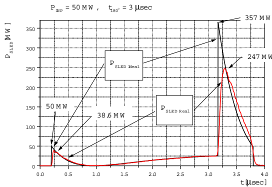
Fig. 4. Pulse shape after power compression system.
