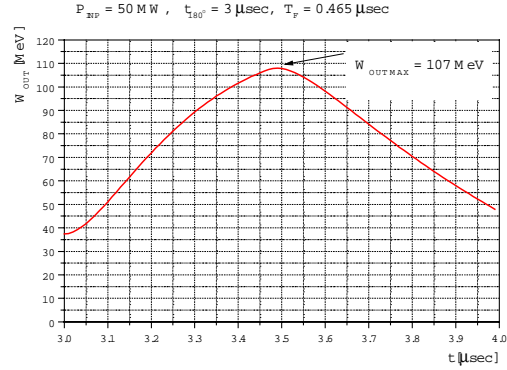
Fig. 5. Beam energy vs. instant of entrance in AS.
